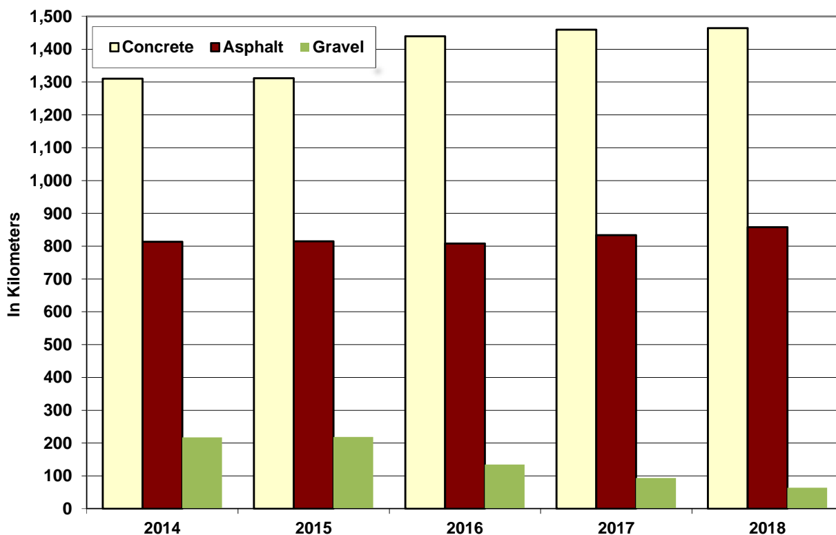
Figure 13.2 EXISTING NATIONAL ROAD LENGTH BY SURFACE TYPE REGION V, 2014 - 2018
