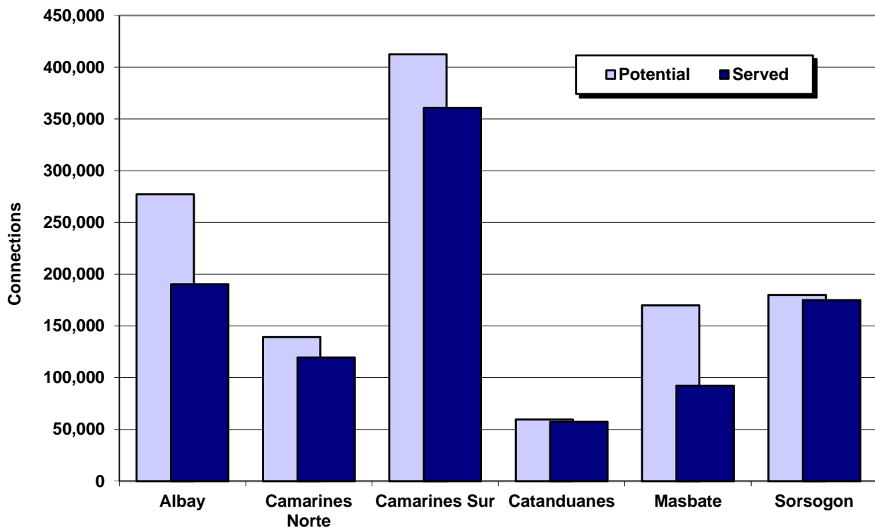
Figure 14.2 ENERGIZATION COVERAGE BY PROVINCE As of December 31, 2018
